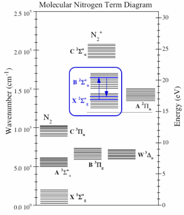
Figure 1: Partial term diagram for molecular nitrogen. The transition of interest is the first negative system; N_2^+ (X^2\Sigma_g^+ (v = v_1)) \rightarrow N_2^+ (B^2\Sigma_u^+ (v = v_2)) \rightarrow N_2^+ (X^2\Sigma_g^+ (v = v_3)) .
