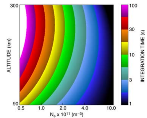
Figure 8: Nomograph for required integration time, as a function of plasma density and altitude, required to recover AMISR plasma measurements with 10% precision.
