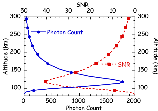
Figure 4: Expected photon count profile (solid) and signal-to-noise ratio (SNR; dashed) measured by proposed auroral lidar system during passage of auroral arcs at 0057 LST on 7 February 1994. The photon count profile represents 300s of integrated lidar echoes measured at 5 km resolution.
